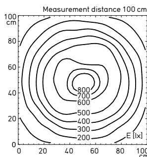
Illuminance 13 W
