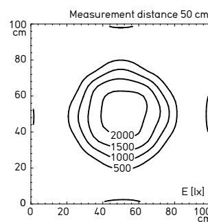
Illuminance based on the example with 70° lens
