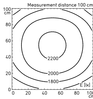
Illuminance 4 x 58 W
