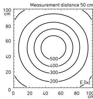
Illuminance 1 x 7 W
