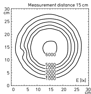
Illuminance 6 W
